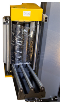
Power pre-stretch film carriage (250%) for greatly improved film efficiency
